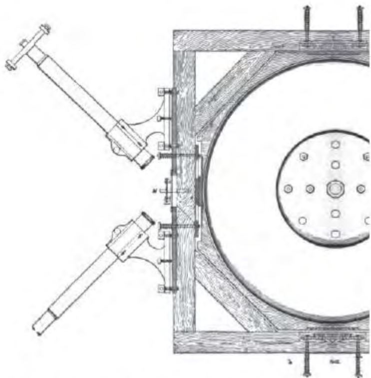
FIG 19 Plan of optical frame with steel disk in position, and frame. G represents one of the pairs of optical glass shims, and part of the fixing of the four mirrors 1234 frame, each mirror held by a brass plate supported, it is pressed by the spring-bolts shown.
